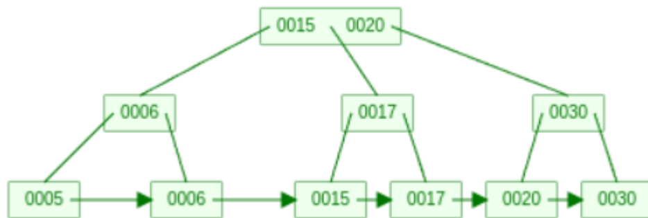
Figure 1 : Initial Tree
